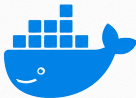
Docker
